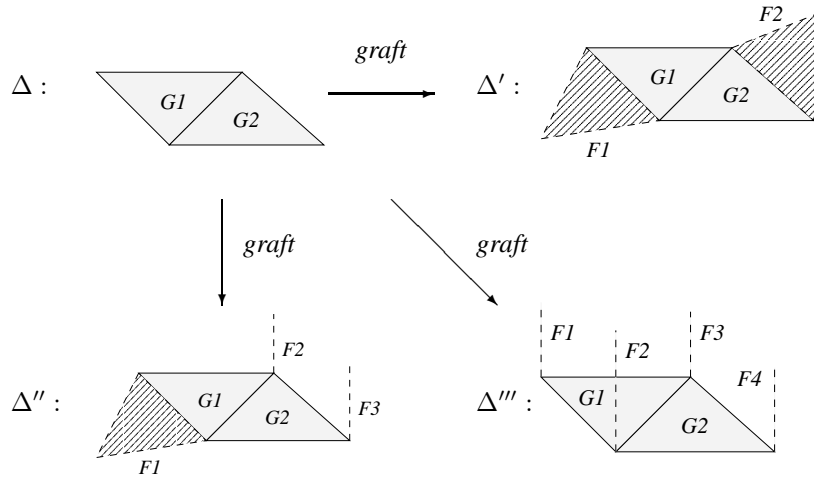
Figure 1: Three different ways of grafting a facet complex \Delta .
